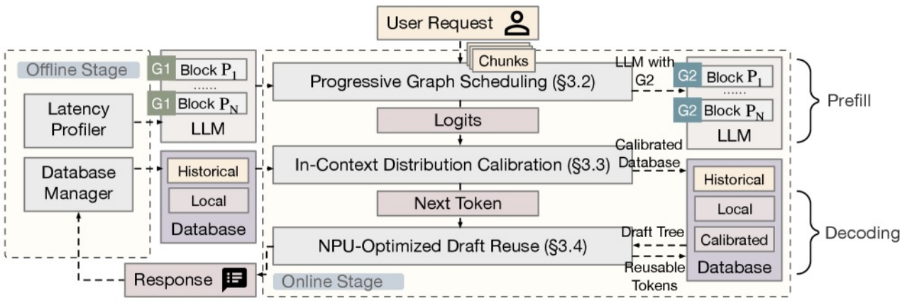
Figure 7. Overview of sd.npu framework. † † :
