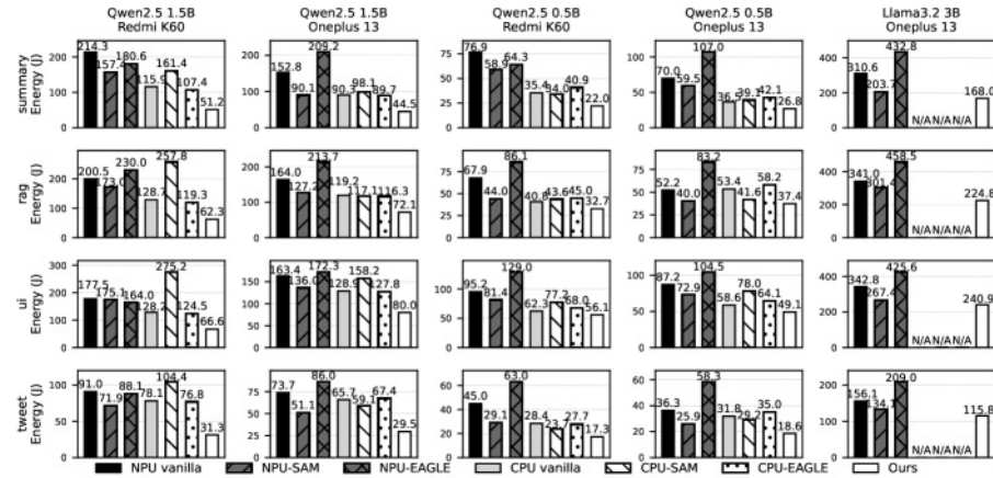
Figure 11. Energy consumption (J) comparison on different datasets, devices and models. \dagger \dagger :
