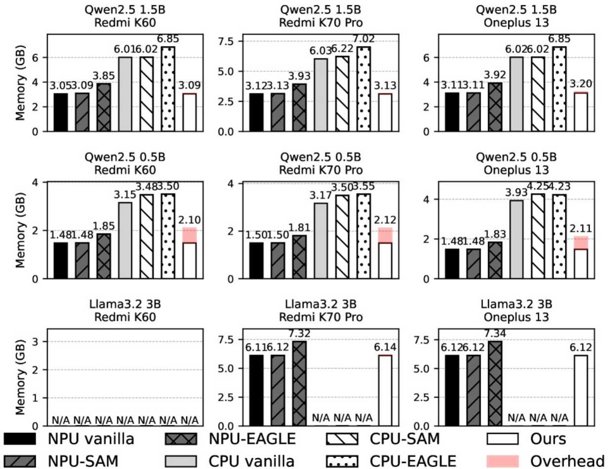
Figure 12. Peak memory comparison (GB) on different devices and models. \dagger \dagger :
