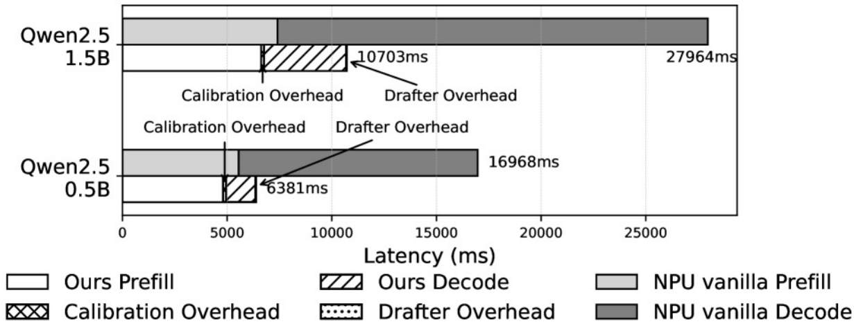
Figure 13. Breakdown of inference latency (ms). † † :
